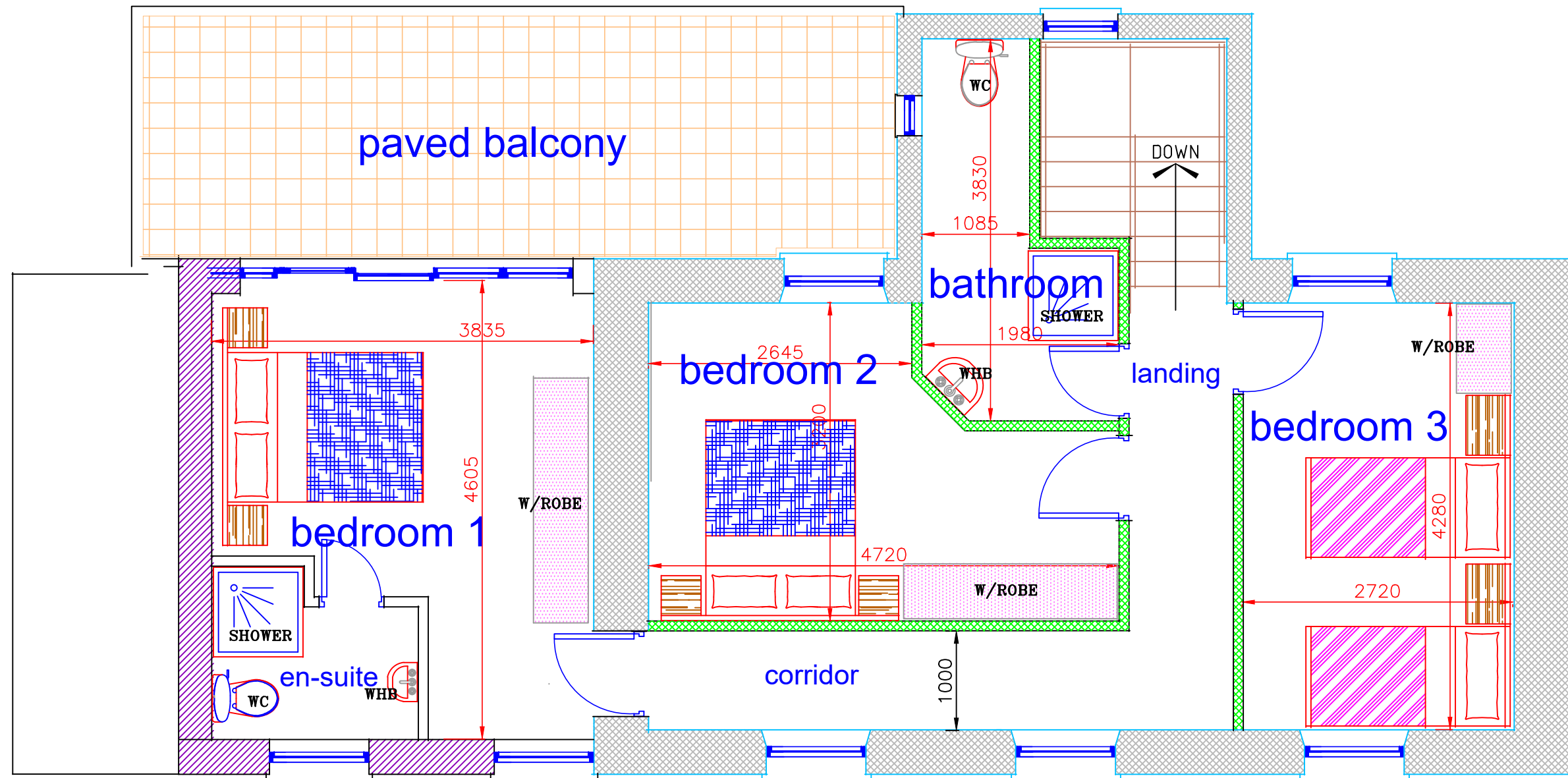
FIRST FLOOR LAYOUT PLAN scale 1:50
